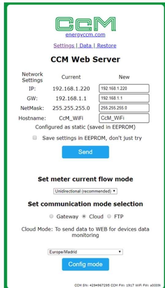
Figura 15 CcM Web Server – Settings
